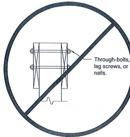
Figure 9. Prohibited Post-to-Beam Attachment Condition.
