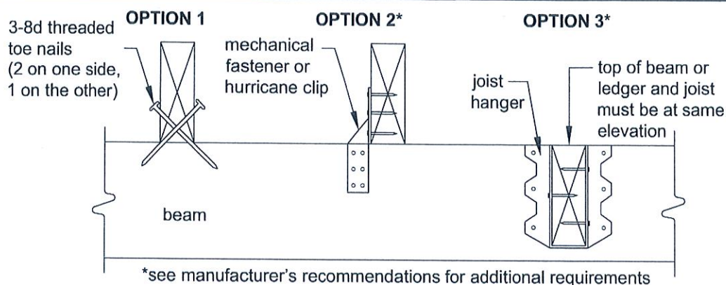
Figure 6. Joist-to-Beam Detail.
