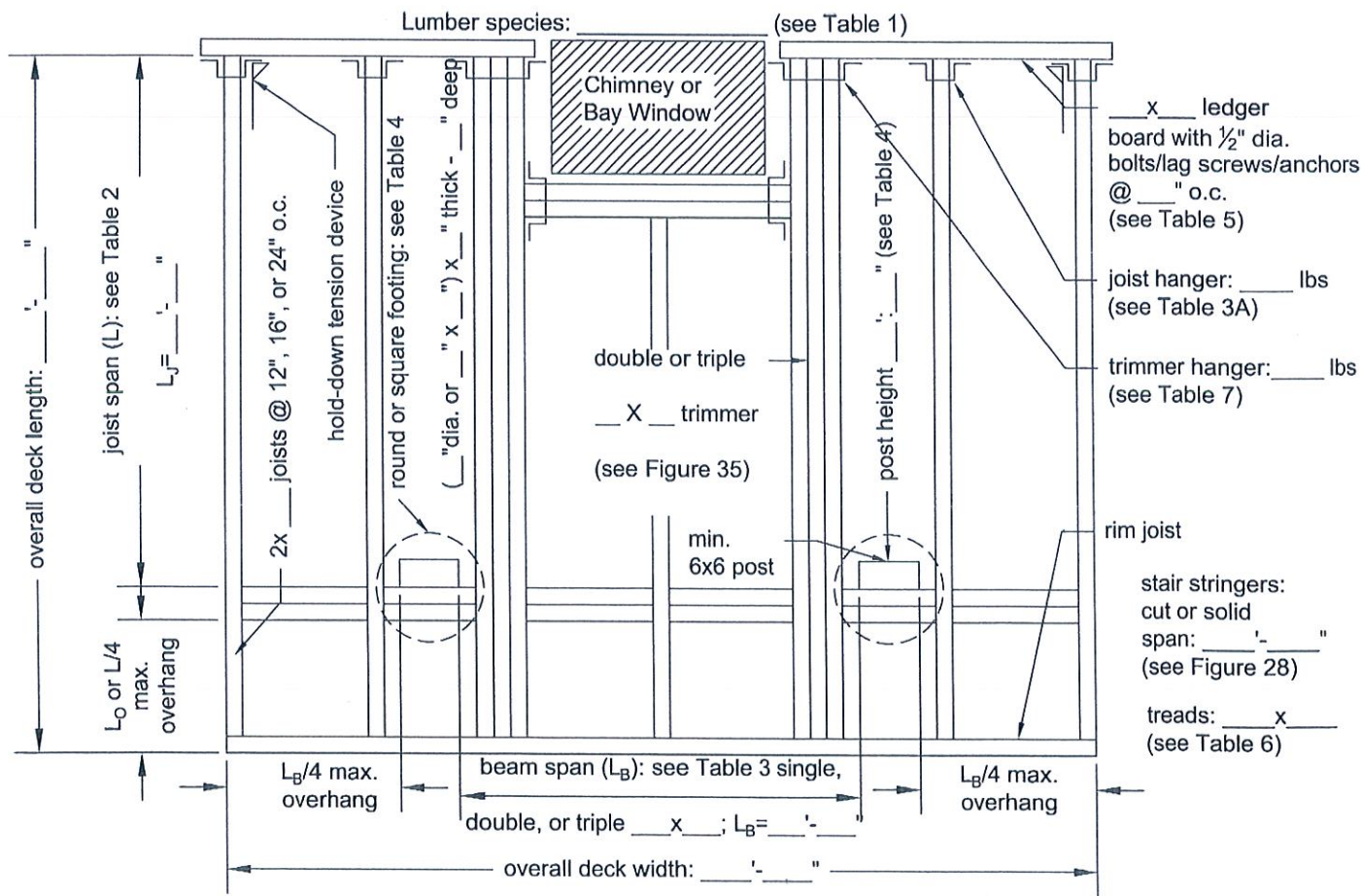
Figure 5. Typical Deck Framing Plan.
