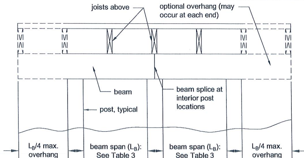
Figure 3. Beam Span.
