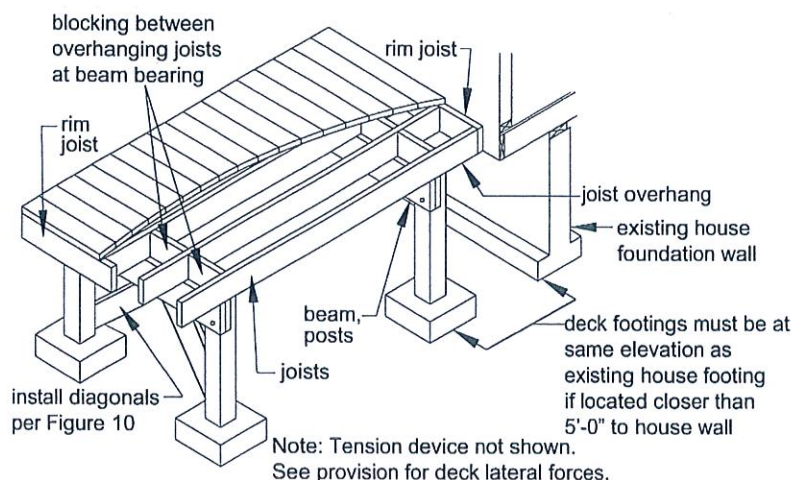
Figure 21. Non-Ledger Deck - For Resisting Vertical Loads.
